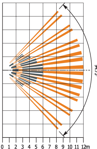
Air2-IR100 Top view
