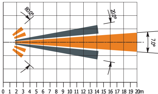
Air2-IR100/C Side view
