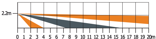
Air2-IR100/C Side view
