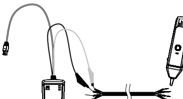
Figure 3. Tracing pairs
