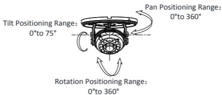
Figure 2.12 3-axis Adjustment
