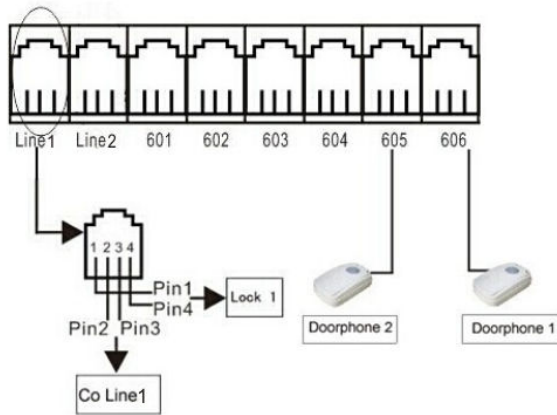
206 Rear View
