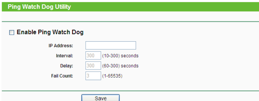
Figure 4-49 Ping Watch Dog Utility
