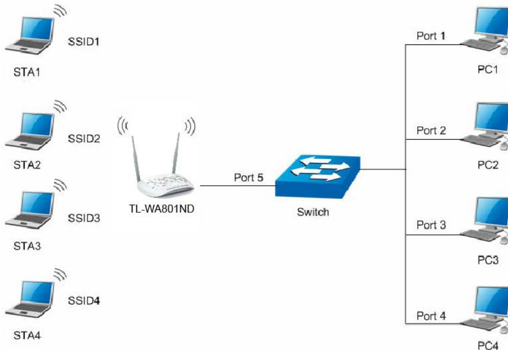
Figure 4-24 Multi-SSID+VLAN
